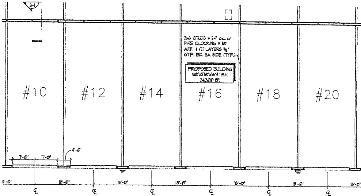
FLOOR PLAN scale: 3/32" = 1'-0"
