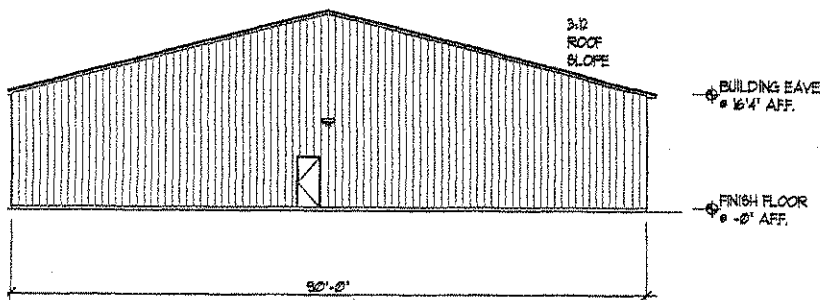
4 SOUTH ELEVATION A-1 scale: 1/16" = 1'-0"
