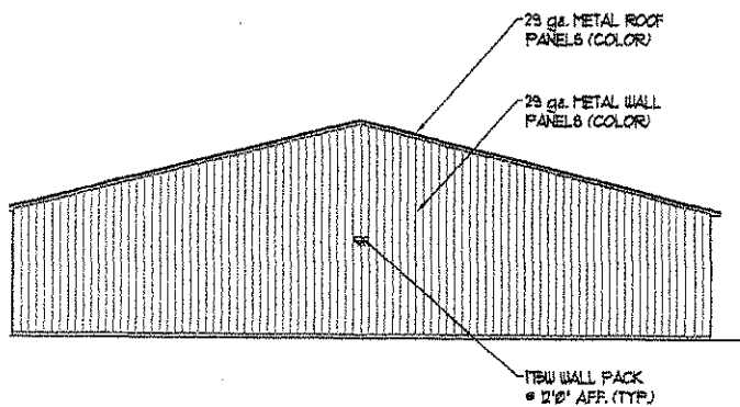
5 NORTH ELEVATION A-1 scale: 1/16" = 1'-0"
